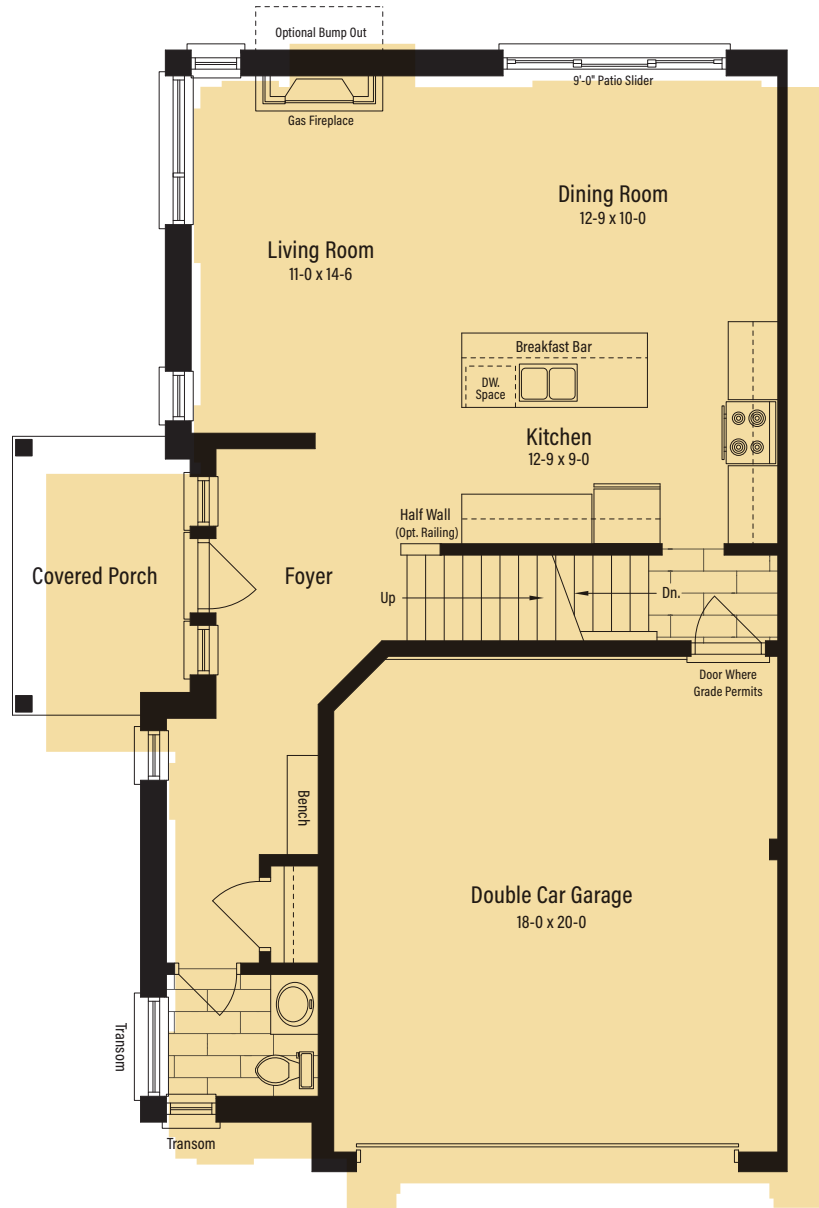
MAIN FLOOR
